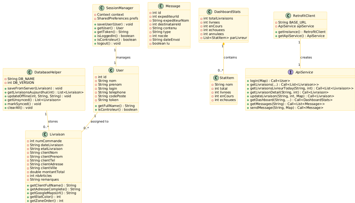
FIGURE 3.1 – Diagramme de Classes – SunDelivery
